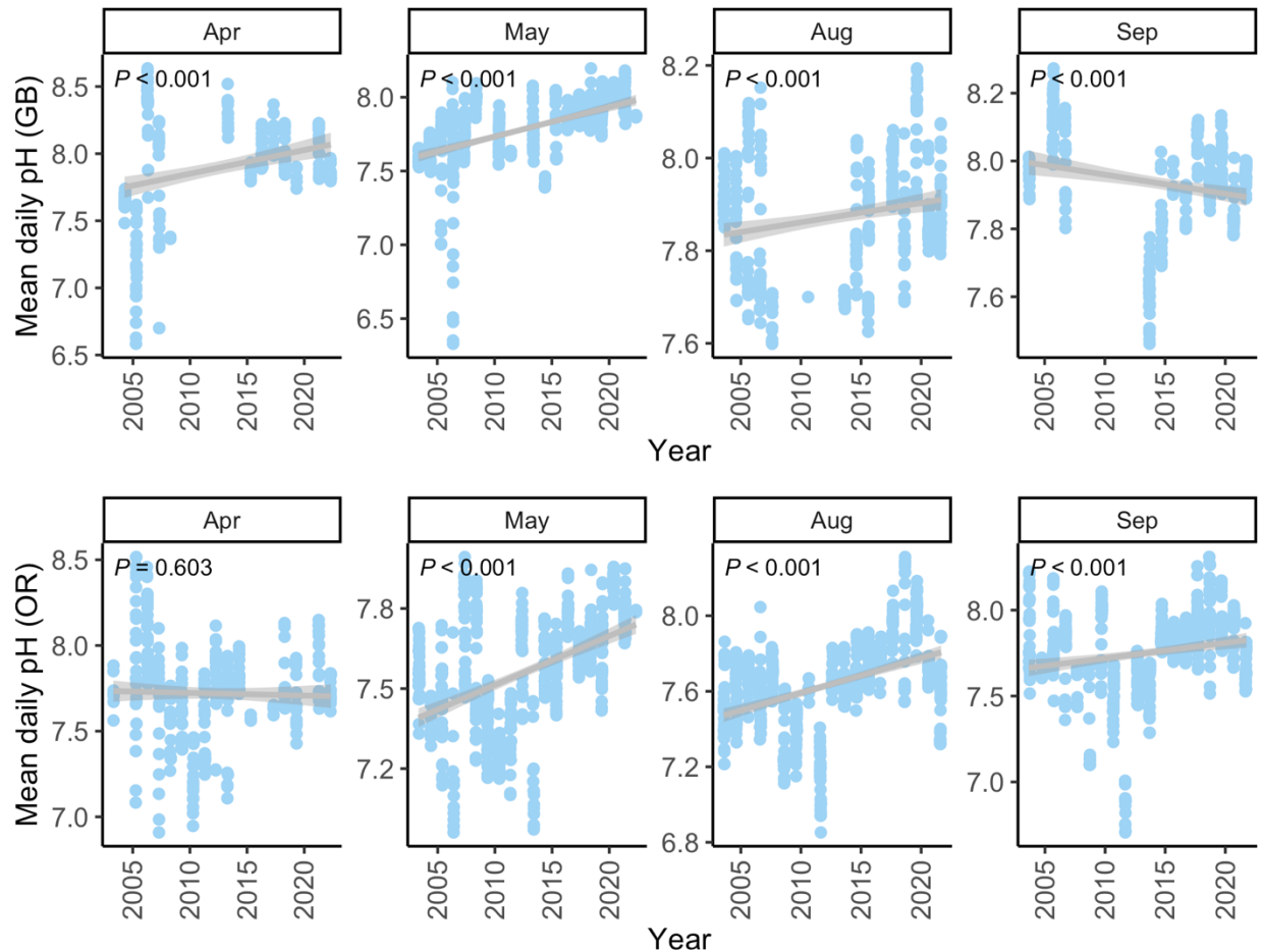
Figure pH-3. Mean daily pH at two representative sites in the Great Bay Estuary: OR = Oyster River and GB = Great Bay, for 4 months spanning the growing season seagrass and seaweed. Each curve represents the line of best fit with a corresponding 95% confidence level interval for predictions from a linear model. Each P value indicates whether the slope of the curve is significantly different from zero.
