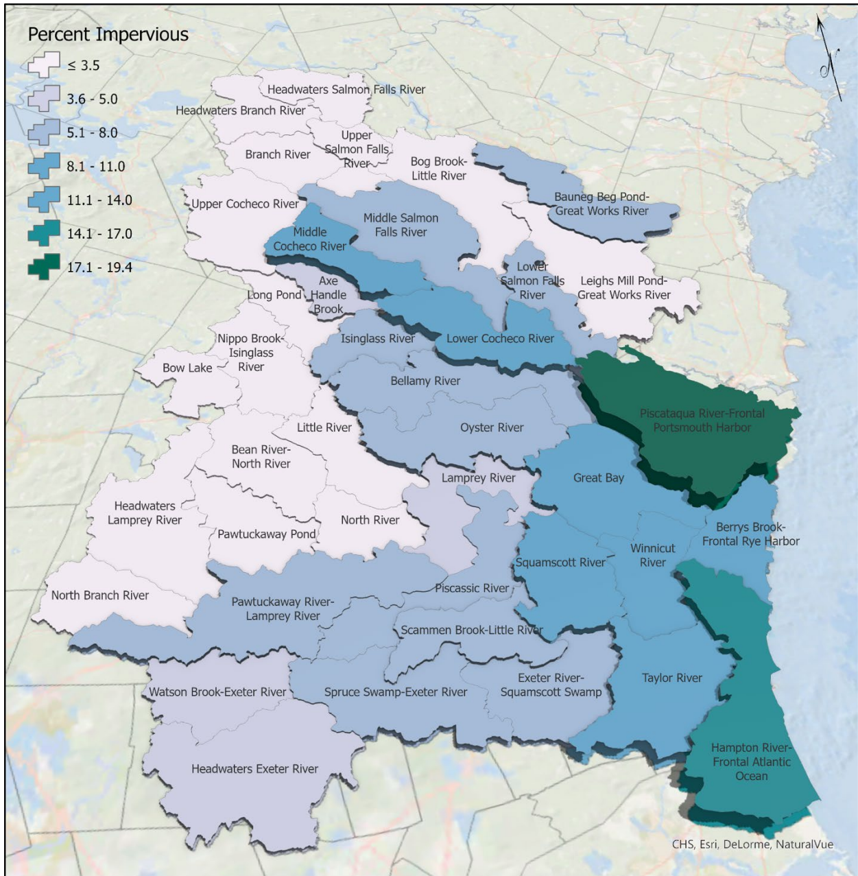
Figure 1.6. Impervious cover by HUC watershed.
