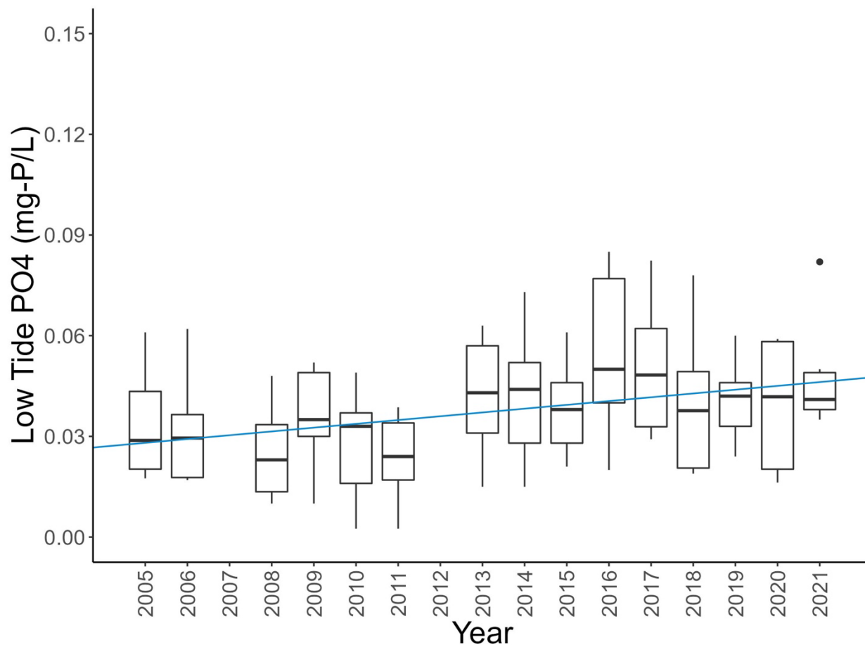
Figure 8.26: Orthophosphate ( \text{PO}_4^{3-} ) at the Squamscott River Station shows an increasing trend over time based on data collected at low tide between 2005 and 2021 and shown as box and whisker plots. Boxes encompass the middle 50% of the data points. The horizontal line in each box is the median and the vertical whiskers encompass values within 1.5*inter-quartile range (99.7% of the data). “Outliers” are shown as individual points. Some years are omitted due to missing data or an insufficient number of measurements that year. Blue line represents significant linear regression through all data points. Data Source: Great Bay National Estuarine Research Reserve and the Jackson Estuarine Laboratory, UNH
